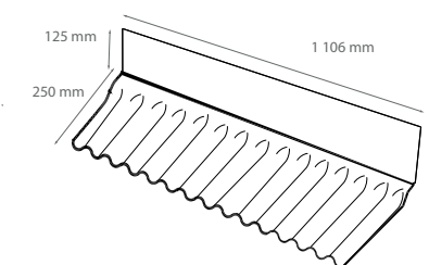
Solin frontal 100°
