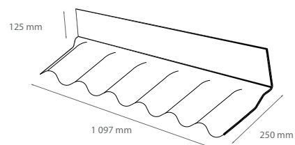
Solin frontal 100°
